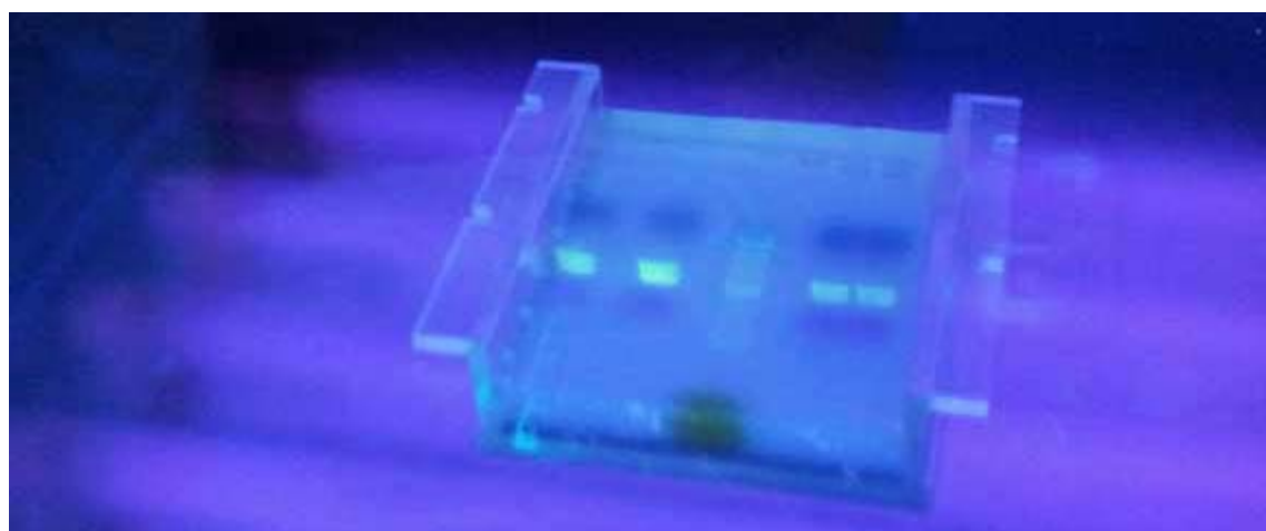
PCR product in an electrophoresis gel prepared for band excision. The excised DNA is subsequently used for cloning and sequencing the targeted gene region.
